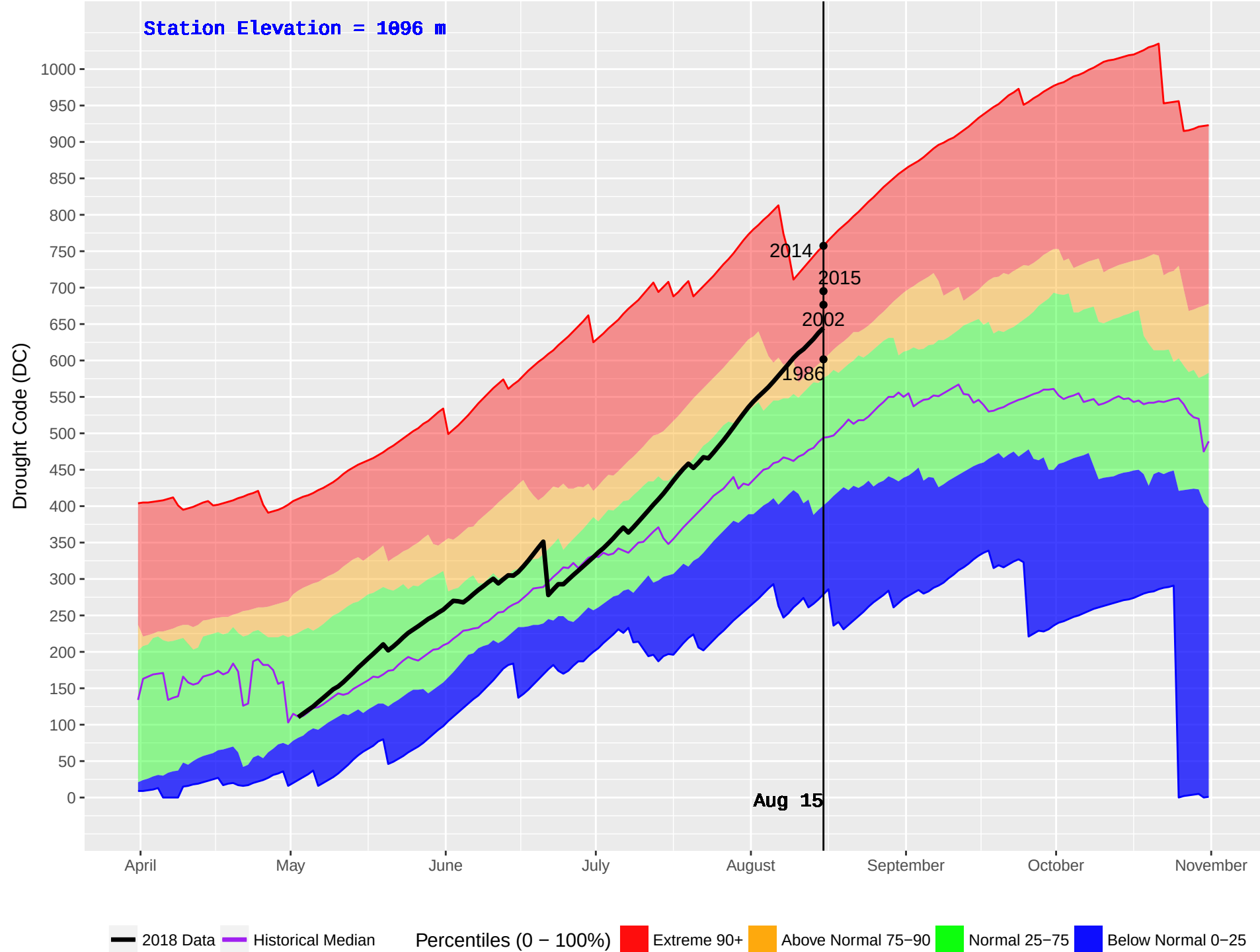
ANAHIM LAKE HUB (213) : Historical (1981–2016) and Current (2018) Daily Drought Code (DC)
